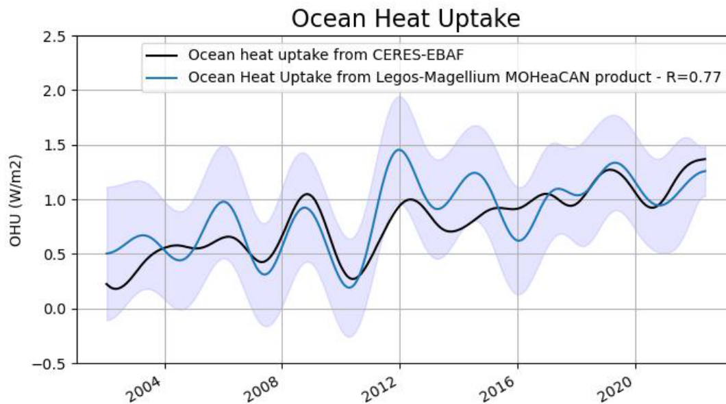
FIGURE 2.6 The Monitoring Ocean Heat Content and earth energy imbalance (MOHeaCAN) (Legos) time series of ocean heat uptake (OHU, blue) and the 90% confidence interval of the Clouds and the Earth's Radiant Energy System Energy Balanced and Filled (CERES EBAF) net radiative flux (EEL, black). Both time series are low-pass filtered at 3 years cut-off time (Lanczos) which removes high-frequency noise related to intrinsic ocean variability. Legos ocean data and CERES Top of Atmosphere (TOA) radiative flux data broadly agree that the Ocean Heat Uptake is increasing over time.
