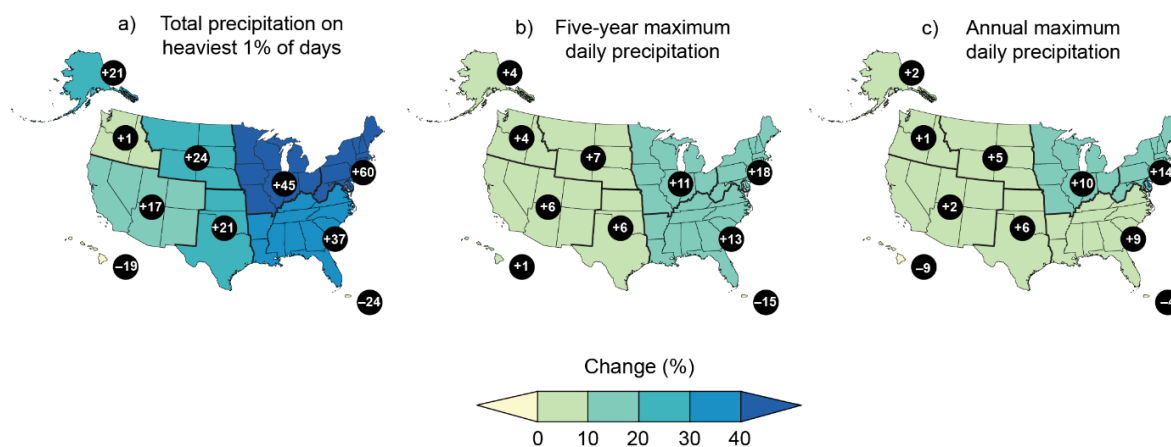
FIGURE 3.2 (Top) Extreme 1-day precipitation events in the contiguous United States, 1910-2023. Percentage of land area of the contiguous states where much greater than normal portion of total annual precipitation has come from single-day precipitation events 1910-2023. The bars represent individual years, while the line is a 9-year weighted average. Data from NOAA NCEI. (Bottom) The frequency and intensity of heavy precipitation events have increased across much of the United States, particularly the eastern part of the United States, with implications for flood risk and infrastructure planning. Maps show observed changes in three measures of extreme precipitation: (a) total precipitation falling on the heaviest 1% of days, (b) daily maximum precipitation in a 5-year period, and (c) the annual heaviest daily precipitation amount over 1958-2021. Numbers in black circles depict percent changes at the regional level. Data were not available for the U.S.-Affiliated Pacific Islands and the U.S. Virgin Islands. Figure credit: NOAA NCEI and CISS NC.
