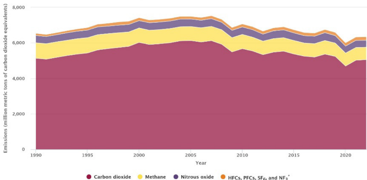
U.S. Greenhouse Gas Emissions by Gas, 1990–2022
