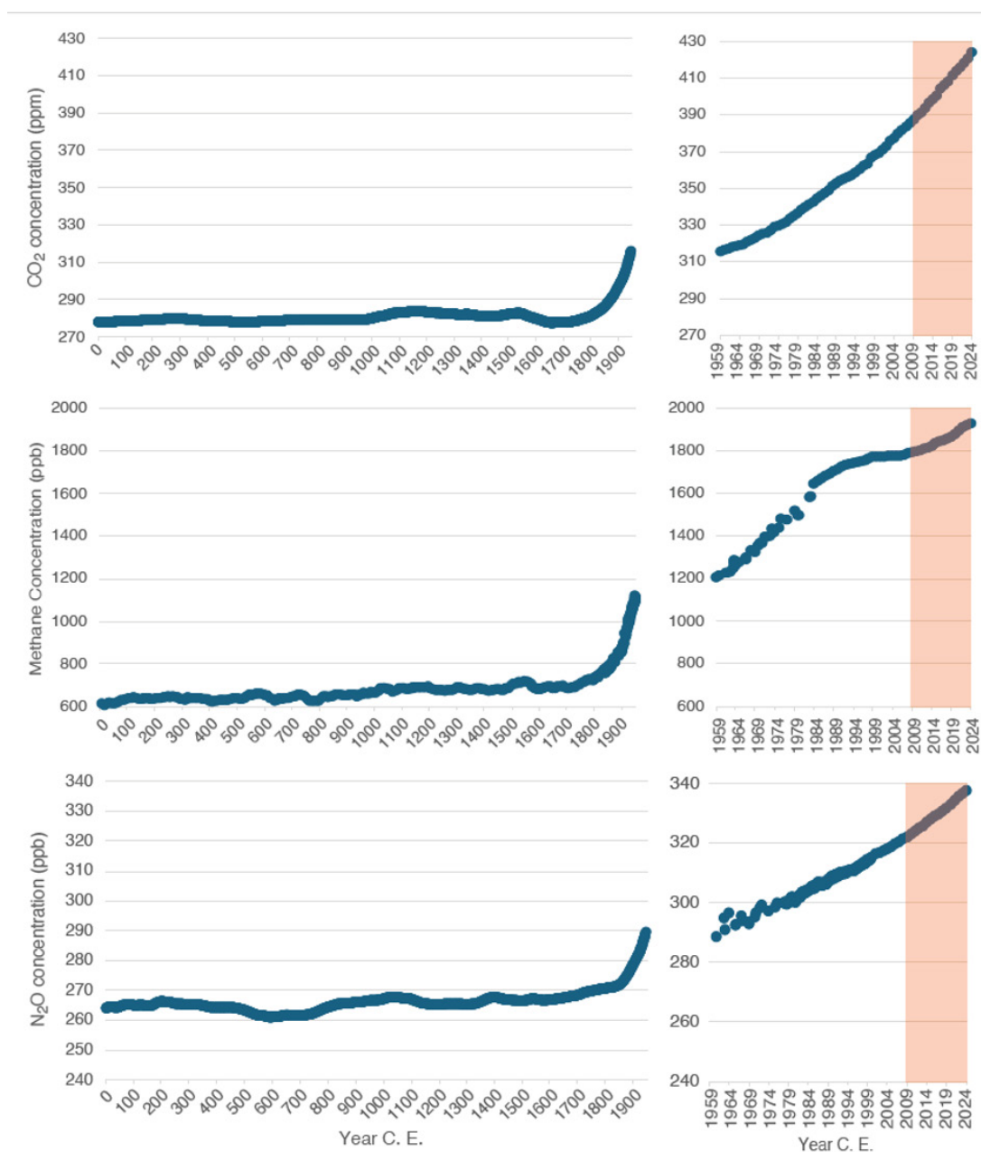
FIGURE 2.5 Global concentrations of the primary human-caused greenhouse gases over the last approximately 2000 years (blue dotted lines), with the shaded areas (orange) indicating the time period since EPA (2009) was published. The timescale (x-axis) for left panel spans 2000 years; the timescale for right spans only the past 65 years.
