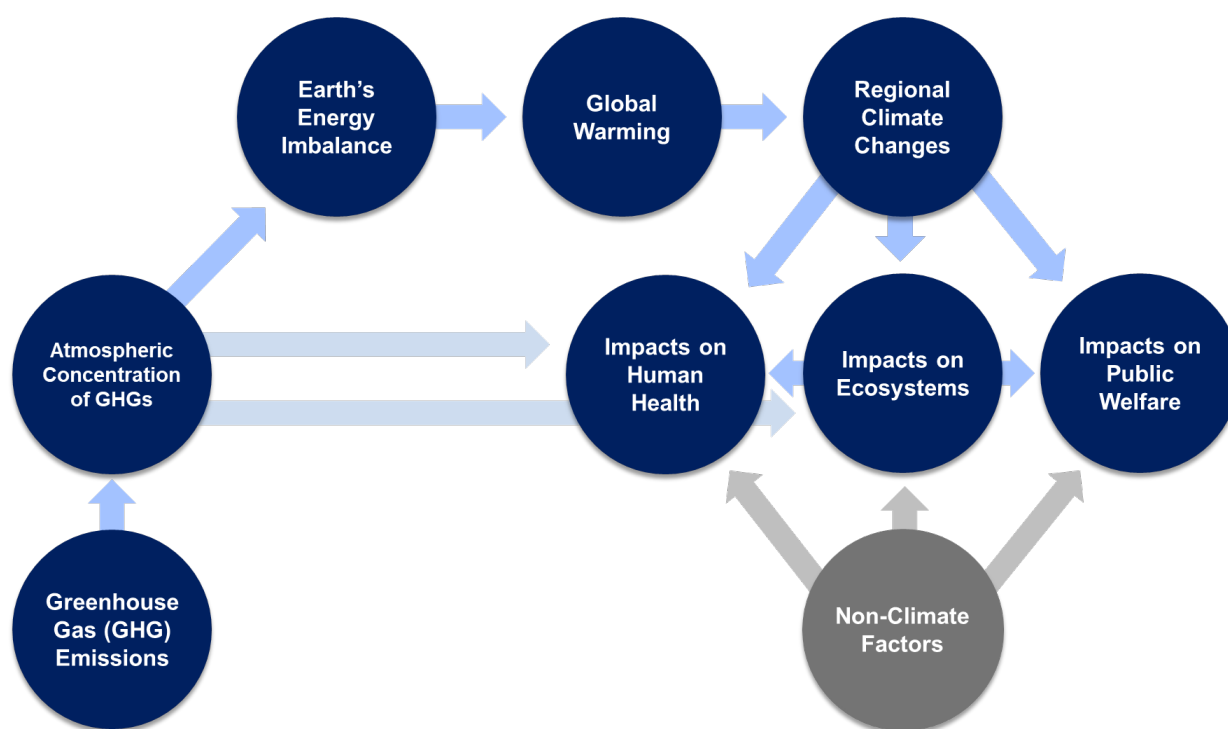
FIGURE 1.1 Schematic of the causal chain from GHG emissions to impacts on human health and public welfare, indicated by the darker blue arrows. The potential direct impacts of GHG emissions on human health (e.g., through contribution to air pollution) and on ecosystems (e.g., changes in ocean chemistry) are indicated by the lighter blue arrows. Non-climate factors, indicated by the grey circle and arrows, include changes in technologies or practices, changes in human systems (e.g., infrastructure, land use), changes in other environmental stressors (e.g., pollution), and other factors that exacerbate or mitigate the impacts of human-caused GHG emissions.
