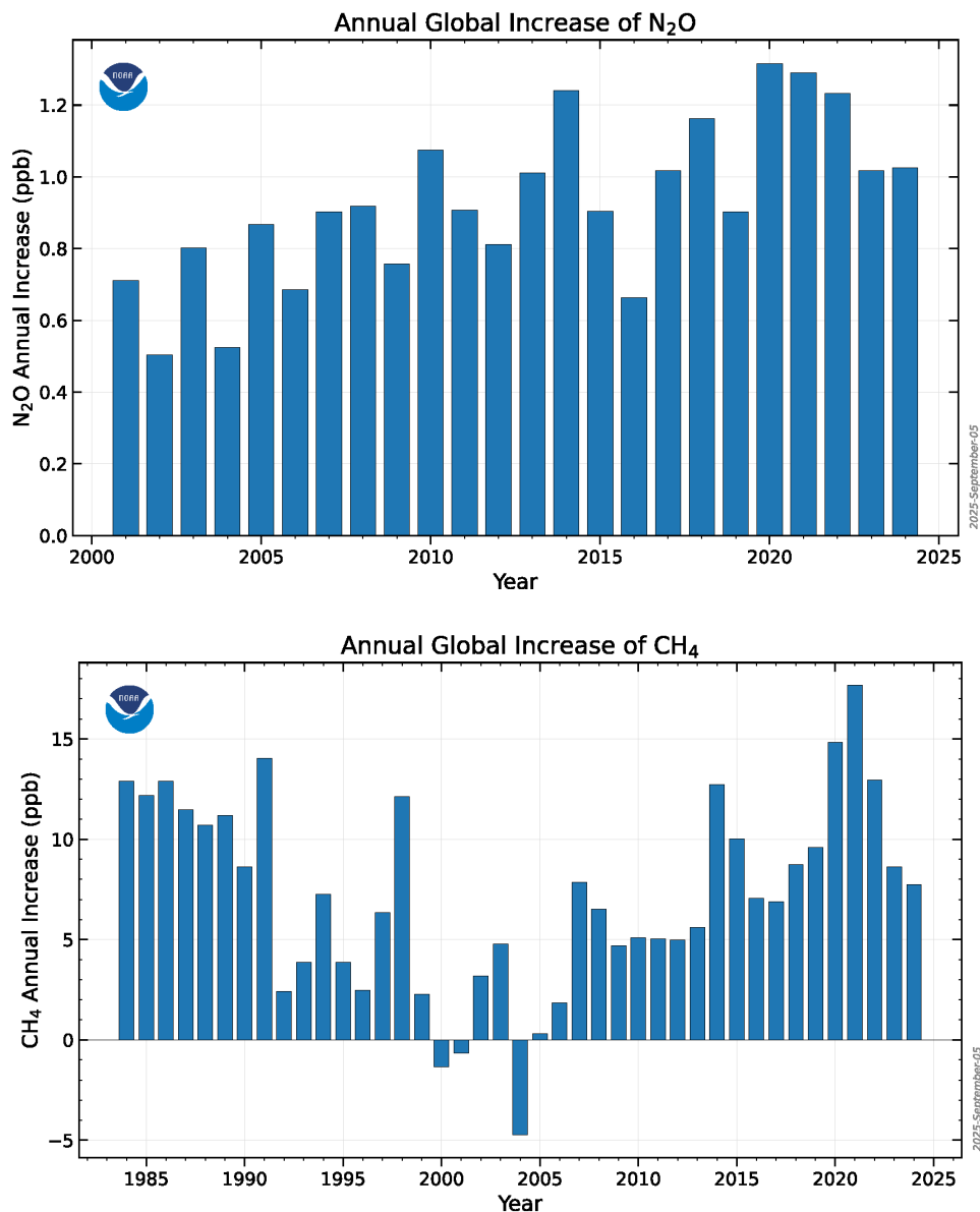
FIGURE 2.4 Annual increases in atmospheric nitrous oxide (N 2 O; top) and methane (CH 4 ; bottom) based on globally averaged marine surface data. The baseline annual atmospheric concentration (0 line) of N 2 O in 2001 is 316.36 parts per billion (ppb) (top) and of CH 4 in 1984 is 1644.84 ppb (bottom). SOURCE: Lan and Dlugokencky, 2022, accessed via NOAA at https://gml.noaa.gov/ccgg/trends_n2o and https://gml.noaa.gov/ccgg/trends_ch4 .
