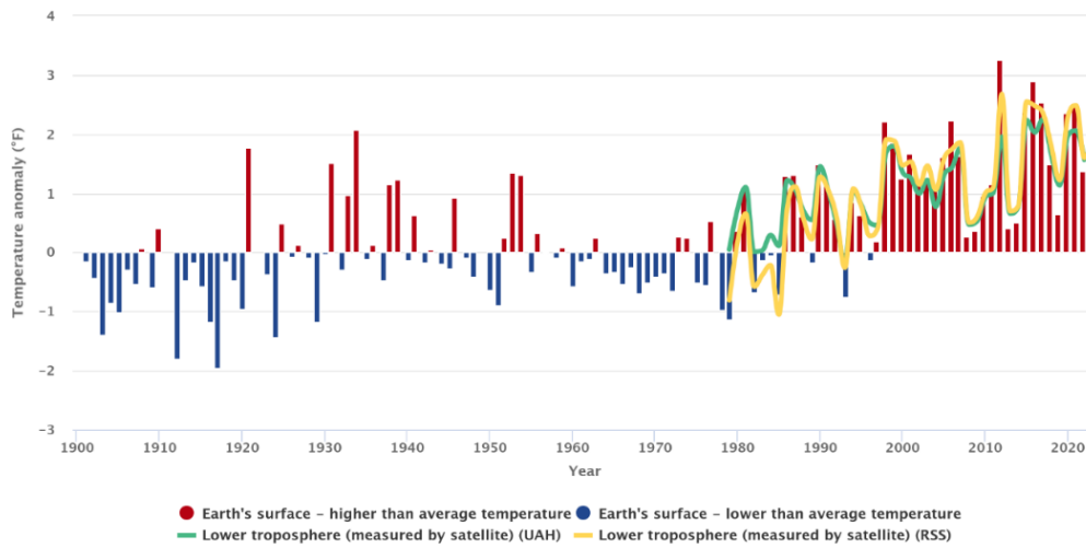
Temperatures in the Contiguous 48 States, 1901–2023
