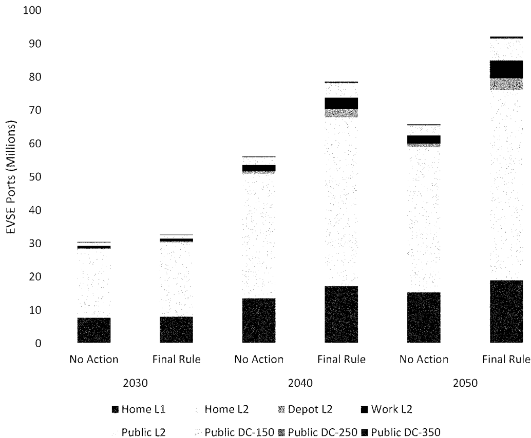
Figure 31: EVSE Port Counts by Charging Location and Type for the No Action Case (Left Side of Each Pair of Bars) and the Final Rule (Right Side of Each Pair of Bars) for Select Years.
