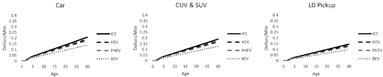
Figure 45: Repair Cost Per Mile (2019 Dollars) for a $35,000 Car, Van/SUV, and Pickup With Various Powertrains by Vehicle Age in Years
