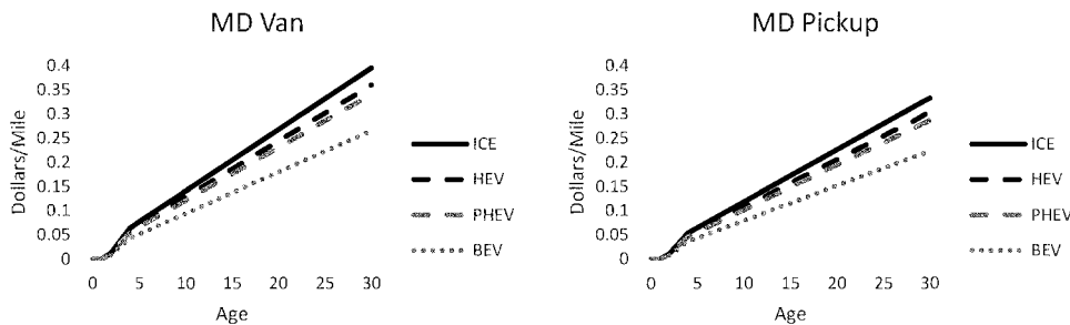
Figure 46: Repair Cost Per Mile (2019 Dollars) for a Medium-Duty Van and Pickup With Various Powertrains by Vehicle Age in Years
