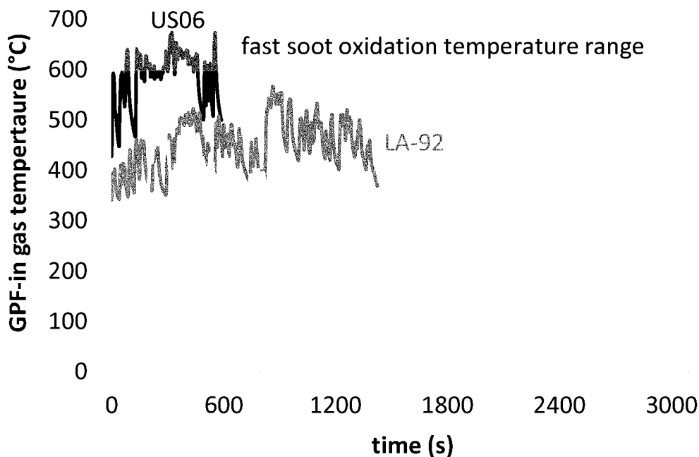
Figure 15: GPF Inlet Gas Temperatures Measured on MY 2022 F250 7.3L Left Engine Bank GPF During Sampled US06, Sampled Hot LA-92, and -7^{\circ}\text{C} FTP Test Cycles
